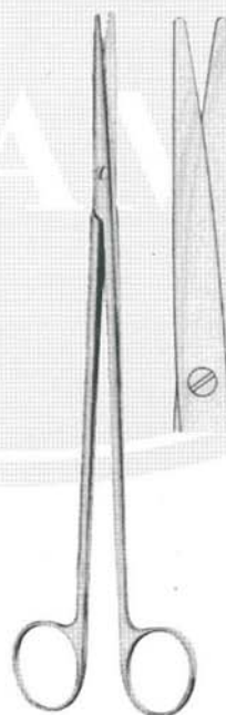
Metzenbaum Fino 22.282.15 150 mm 22.282.18 180 mm 22.282.20 200 mm 22.282.23 230 mm 22.286.15 TC 150 mm 22.286.18 TC 180 mm 22.286.20 TC 200 mm 22.286.23 TC 230 mm
