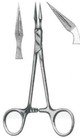
24.822.13 Stiegletz 135 mm 24.823.13 straight curved
