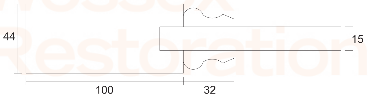
Section Through Stile
