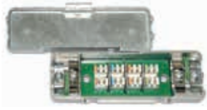
Cable connector Cat. 7 IP20
