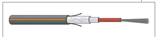
FO Outdoor ZGGT HP / A-DQ(ZN)B2Y HighP, up to 24 fibres
