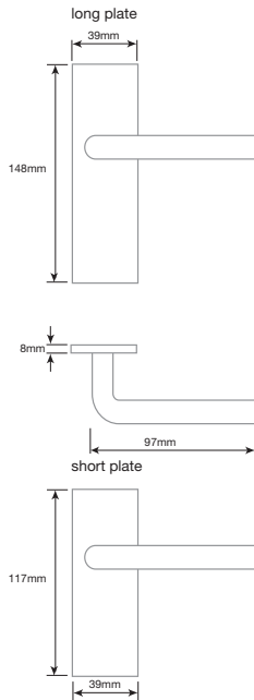
Privacy Short Plate JV131PR EB
