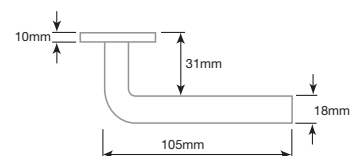
Latchset JV661PB JV661PC JV661SC
