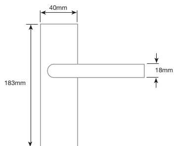
Lockset JV660PB JV660PC JV660SC
