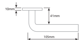
Latchset JV191AB JV191PC JV191SC
