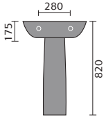
bordeaux 55cm basin 1th full pedestal
