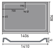
1400 x 800mm rectangular
