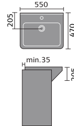
provence 55cm semi recessed basin
