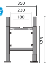
wall hung frame (PORIMWF)
