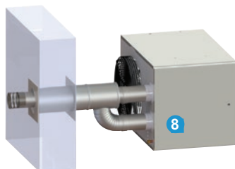
Concentric wall duct C12 maximum length : 6m
