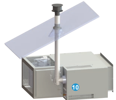
Sealed roof chimney B22 maximum length : 8m
