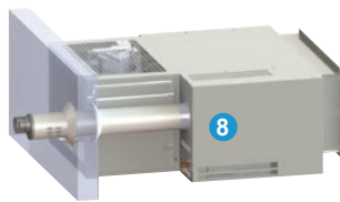
Concentric wall duct C12 maximum length : 6m
