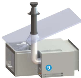
Concentric roof duct C32 maximum length : 6m
