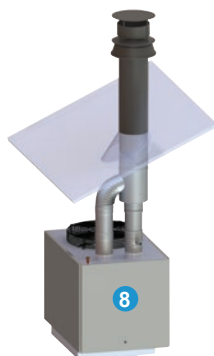
Concentric roof duct C32 maximum length : 8m
