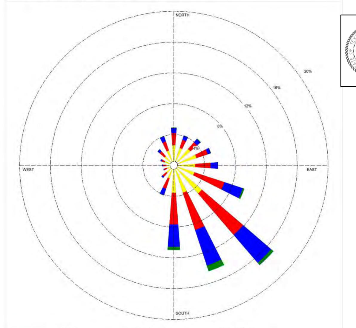
WIND ROSE PLOT Station #12960 - HOUSTON/INTERCONTINENTAL ARPT, TX
