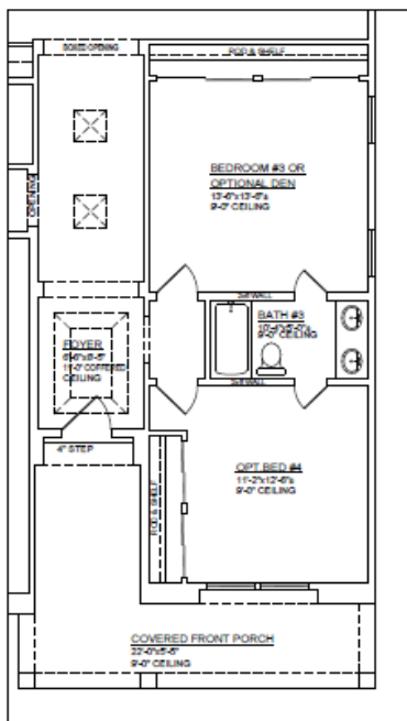
FLOOR PLAN - W/ OPT. 4TH BEDROOM Approx 2301 sq/ft
