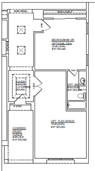
FLOOR PLAN - W/ OPT. FLEX SPACE Approx 2379 sq/ft
