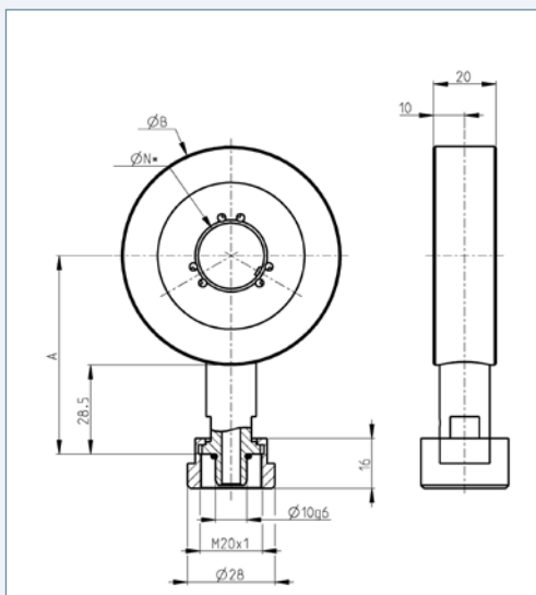
AG200-S3-3-150; diameter 3^* \leq \varnothing N \leq 150 mm
