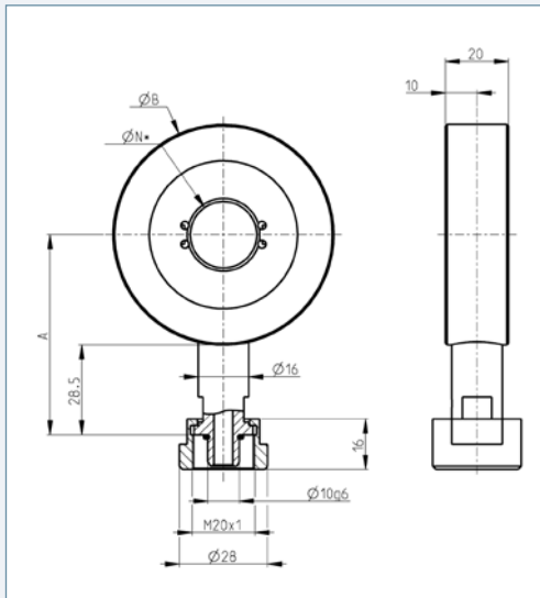
AG200-S2-3-150; diameter 3^* \leq \varnothing N \leq 150 mm
