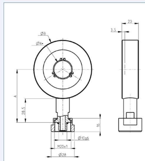
AG200-TP3-3-150, diameter 3^* \leq \varnothing N \leq 150 mm
