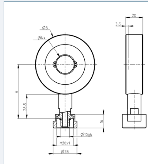
AG200-TP2-3-150; diameter 3^* \leq \varnothing N \leq 150 mm
