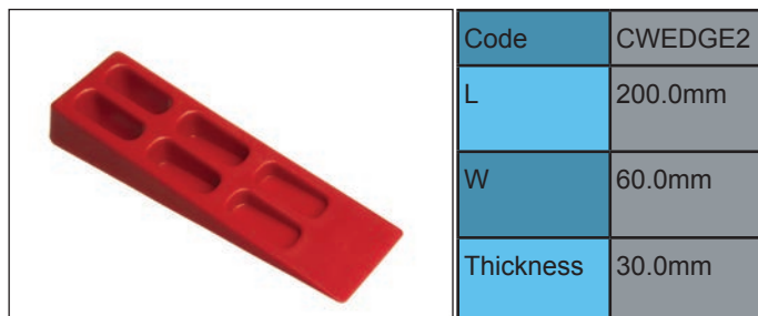
PLASTIC WEDGE MEDIUM
