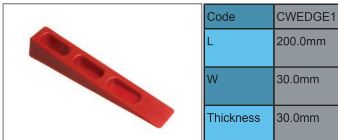
PLASTIC WEDGE SMALL
