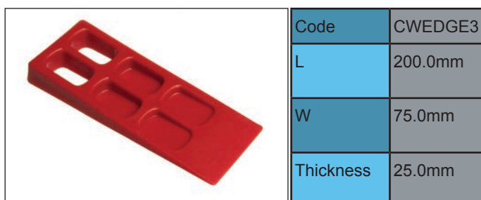
PLASTIC WEDGE LARGE
