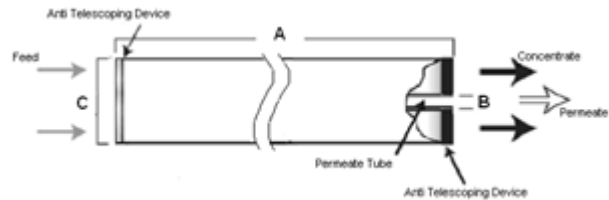
Figure 1b: Element Dimensions Diagram – Female
