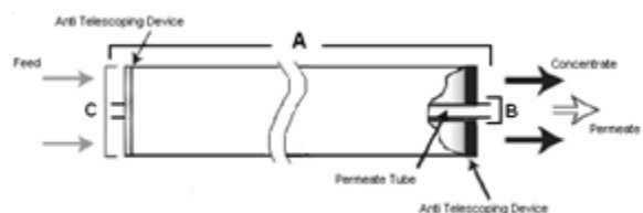
Figure 1a: Element Dimensions Diagram – Male
