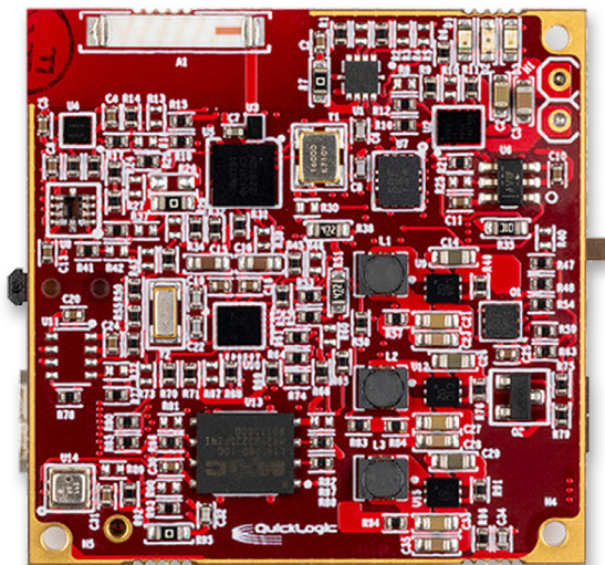
QuickLogic Chilkat HDK (34.29mm x 34.29)
