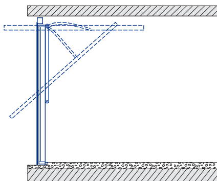
Canopy Operating Gear
