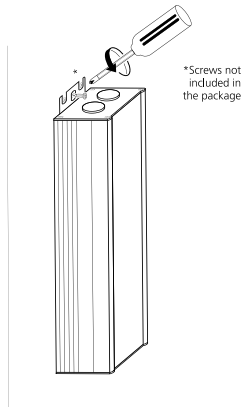
Vertical installation
