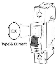
MCB example
