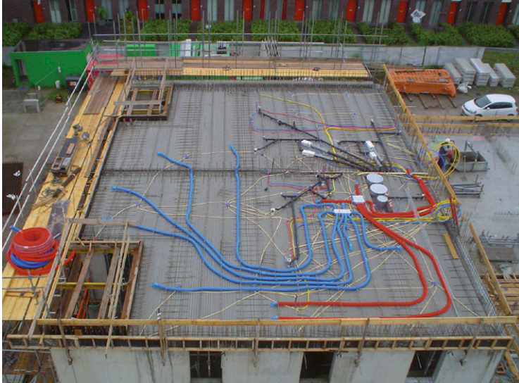
Layout suggestion, Hybalans+ system
