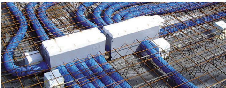
Suggested layout showing air distribution manifold for air supply
