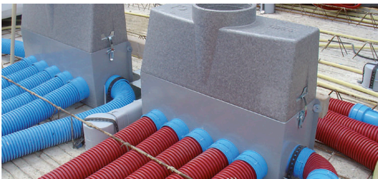
Suggested layout showing air distribution manifold for balanced ventilation
