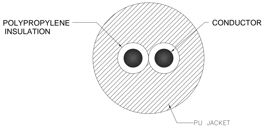
GEOPHONE LEADER CABLE (2 CORE)
