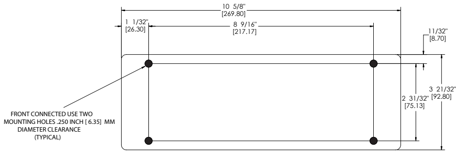
10 POLE BASE
