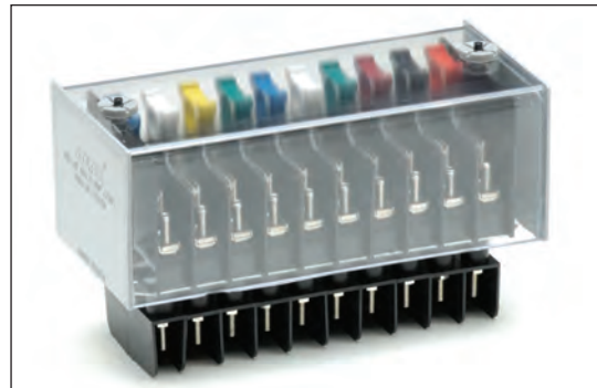
Nonslotted, back-connected clear cover – The nonslotted covers for back-connected switches fit flush with the panel because all wiring exits at the rear of the test switch
