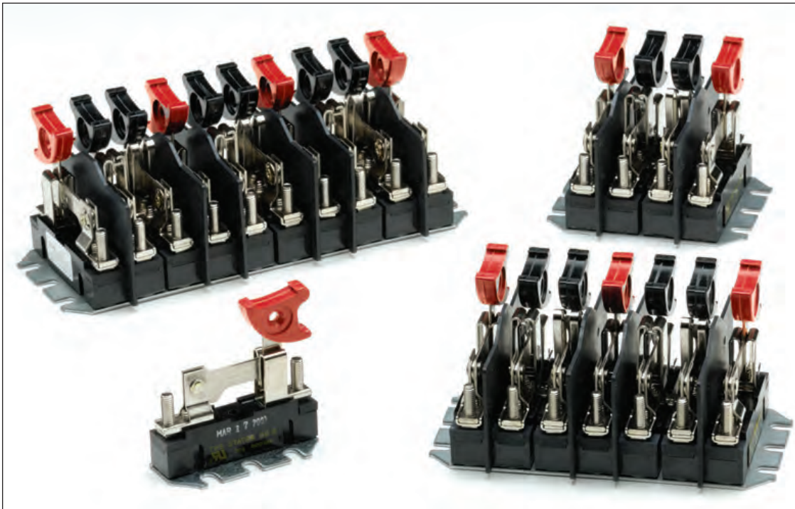
Space-saving miniaturization means full test capability; yet, a Type MTS 10-pole switch requires just 7 inches of mounting space. Unit-pole construction permits virtually any pole arrangement from 1 to 52 poles mounted on a single base.
