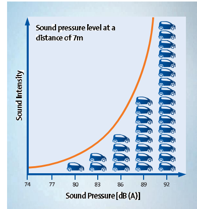
If two cars each produce 80dB, their joint noise level is not 160 dB, rather it is 83dB.
