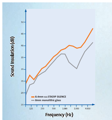
Performance of SGG STADIP SILENCE in a double glazed unit
