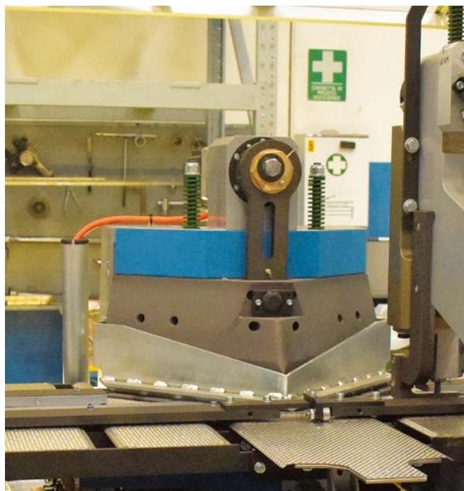
Figure 2. V-Notch
