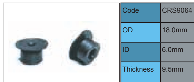
NECKAR
