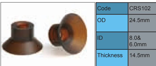
MULLER MARTINI #0020.1927 - ACLA PU VERSION
