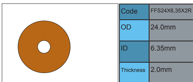
MULLER MARTINI COLLATOR #0020.1907 OLD CODE FS76
