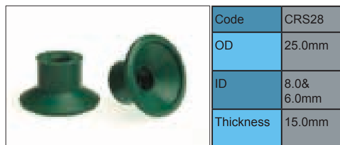
MULLER MARTINI #0020.1910 CRS28B - BLACK
