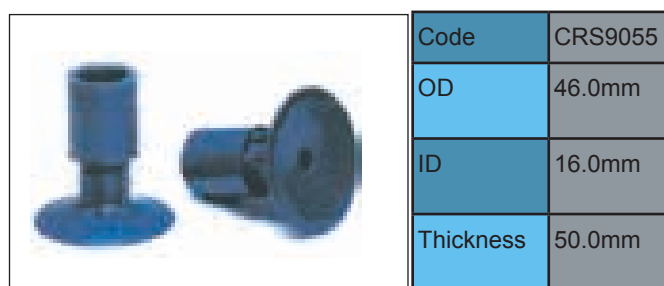
MAILANDER / CRABTREE
