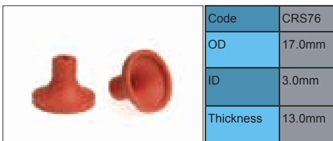
SHERIDAN CRS76S - ALTERNATIVE
