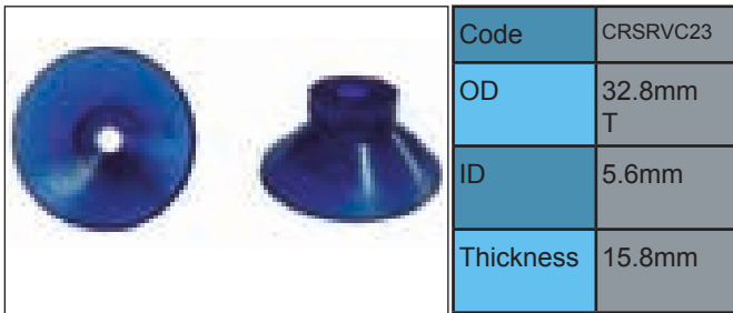
MISCELLANEOUS
