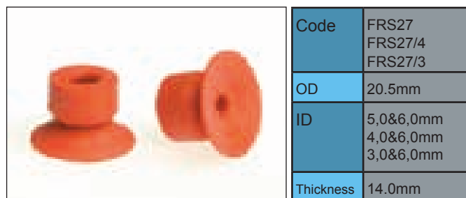
MULLER MARTINI COLLATOR #0020.1903 (RS 27 ID:5.0&6.0mm) MULLER MARTINI COLLATOR #0020.1902 (RS 27/4 ID:4.0&6.0mm) MULLER MARTINI COLLATOR (RS 27/3 ID:3.0&6.0mm)
