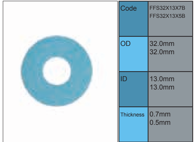
KOMORI #K6223212081 (FFS32X13X7B0) OLD CODE FS17 KOMORI #K6223212051 (FFS32X13X5B0) OLD CODE FS16
