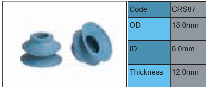
SHOEI COLLATOR - SOFT
