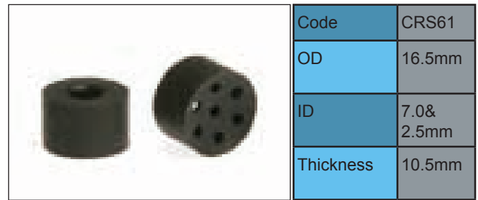
MULLER MARTINI #0020.1916 #0020.1912 - 7 HOLES
