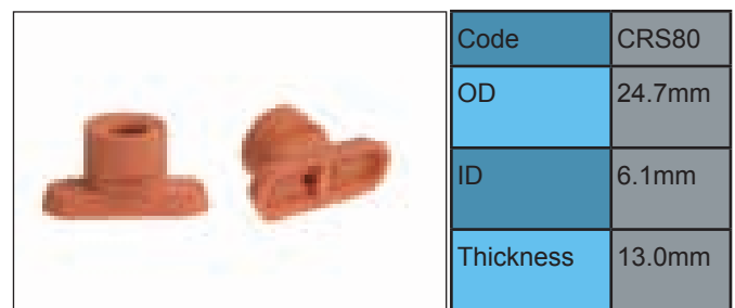
MULLER MARTINI #0020.1914 - 2 HOLES
