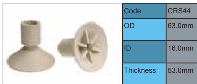
MAILANDER / CRABTREE
