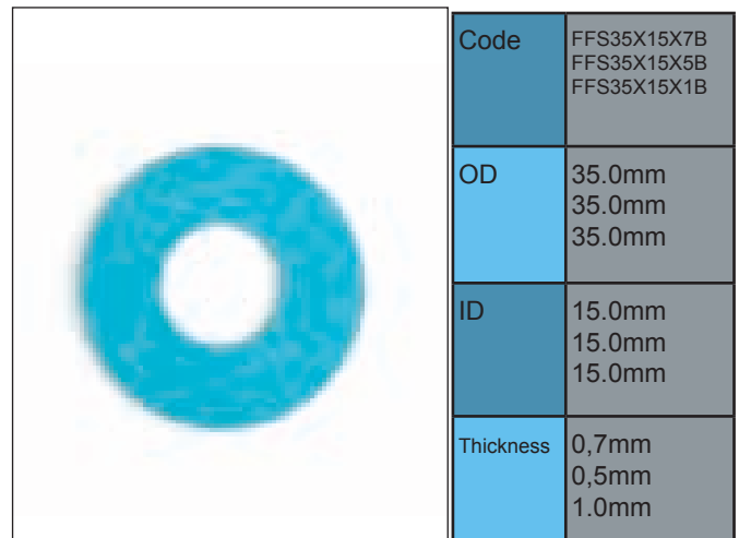
KOMORI #K4441679014 (FFS35X15X7B) - OLD CODE FS23 KOMORI #K6223414051(FFS35X15X5B) - OLD CODE FS22 KOMORI (FFS35X15X1B) - OLD CODE FS24
