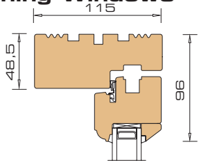
1 Vertical section head / -sash
