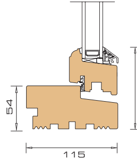
4 Vertical section sill / -sash
