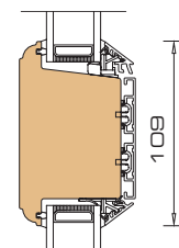
Vertical section 109 mm rail
