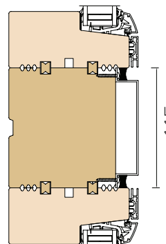
180° linking post
