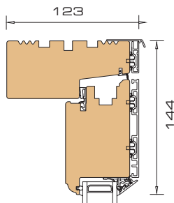
1 Vertical section head / -sash
