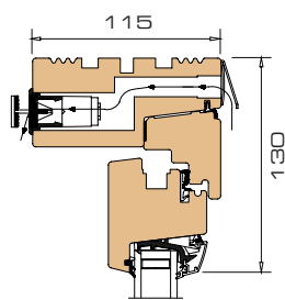
1 Vertical section head / -sash with vent
