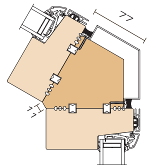
60° corner post
