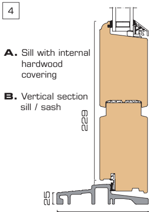
(outward opening)
