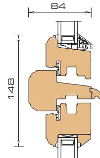
5 Vertical section transom / sashes
