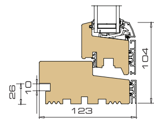
4 Vertical section sill / -sash
