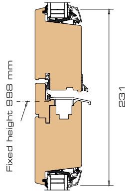
6 Vertical section rebated sashes
