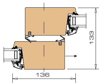
4 Horizontal section rebated sashes
