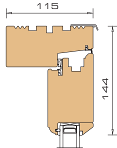
1 Vertical section head / -sash
