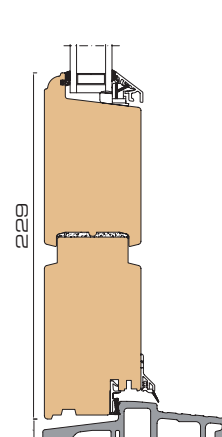
(inward opening)
