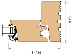
5 Horizontal section locking side
