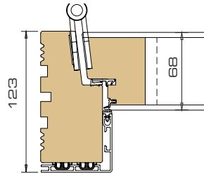
6 Vertical section rebated sashes
