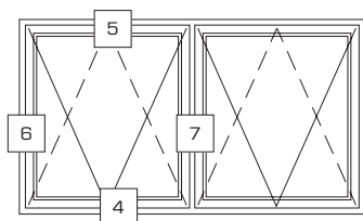
Type B27.00 - 27.10
