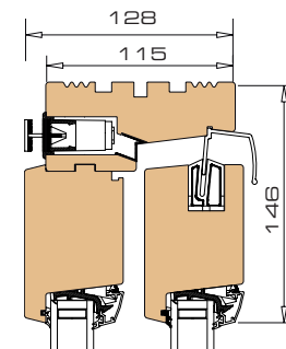
1 Vertical section head / -sash with vent
