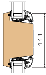
Vertical section 111 mm rail
