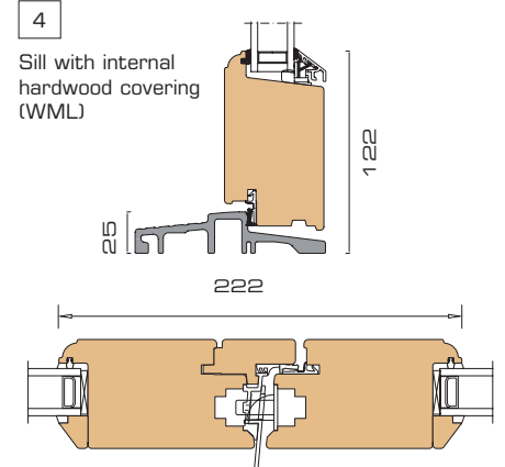
5 Horizontal section rebated sashes
