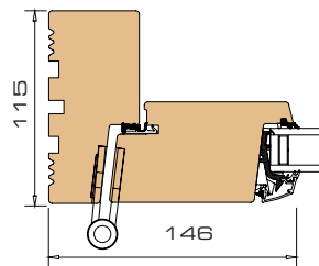
2 Horizontal section hinge side
