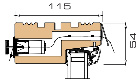
1 Vertical section head with vent
