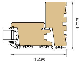
5 Horizontal section locking side
