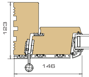
2 Horizontal section hinge side with vent
