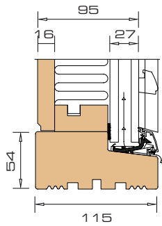
Vertical section sill
