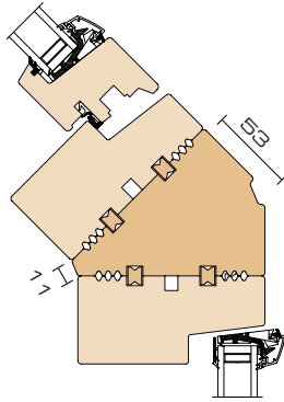
45° corner post
