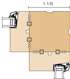
90° corner post
