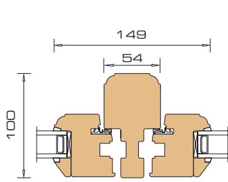
3 Horizontal section mullion / -sashes
