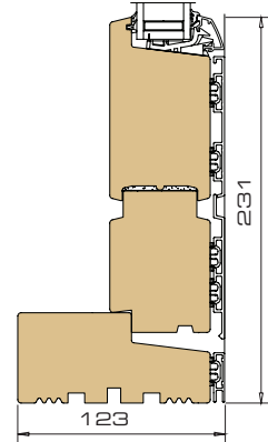
3 Vertical section sill with rails
