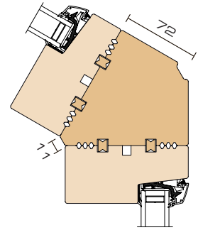
60° corner post
