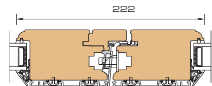
5 Horizontal section rebated sashes
