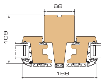
3 Horizontal section mullion / -sashes
