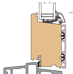
3 Sill with internal hardwood covering. Standard on terrace doors, optional for entrance doors. (WML)
