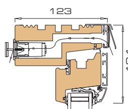
5 Vertical section head / -sash with vent
