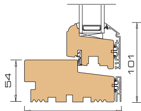
4 Vertical section sill / -sash
