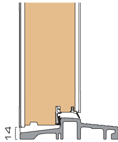
4 Vertical section sill / door plate
