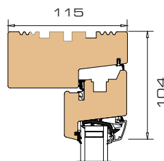
1 Vertical section head / -sash
