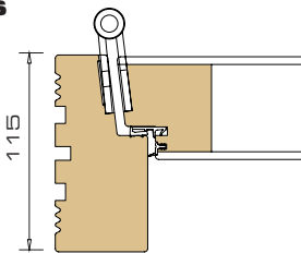
1 Vertical section head / door plate
