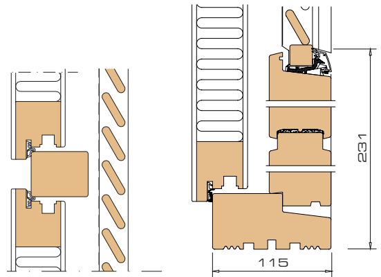
4 Vertical section sill with rails
