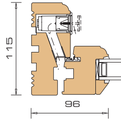
2 Horizontal section jamb / -sash with vent
