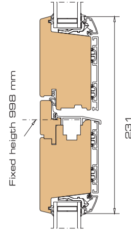
6 Vertical section rebated sashes
