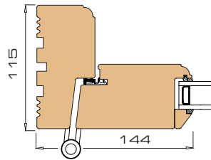
2 Horizontal section hinge side
