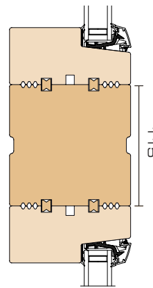
180° linking post
