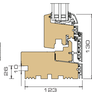
3 Vertical section sill / -sash
