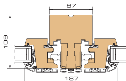
7 Horizontal section mullion / -sashes
