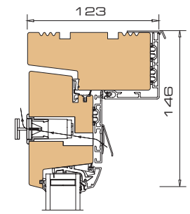
5 Vertical section head / -sash with vent
