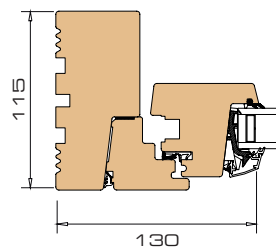
2 Horizontal section hinge side
