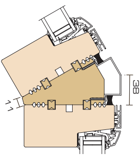
30° Corner post
