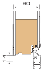
4 Vertical section bottom rail / door plate
