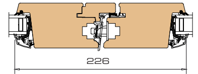
4 Horizontal section rebated sashes
