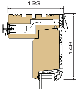
1 Vertical section head with rail with vent
