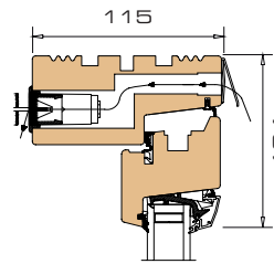
5 Vertical section head / -sash with vent
