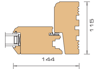
3 Horizontal section locking side
