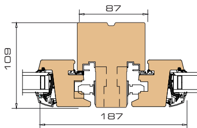
7 Horizontal section mullion / -sash
