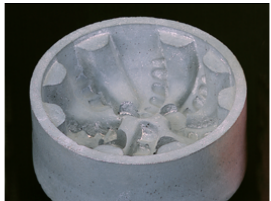
Ceramacast™ 673 mold for down-hole drill bit.
