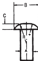
STANDARD UNIVERSAL HEAD ALUMINUM RIVETS
