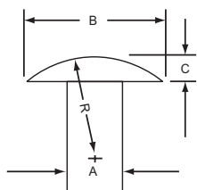
STANDARD BRAZIER HEAD ALUMINUM RIVETS
