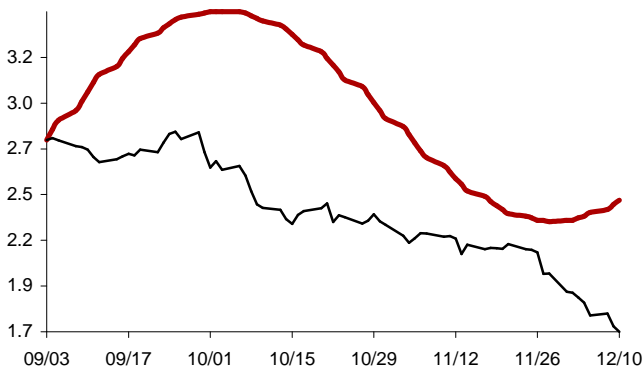
Chart 5: Forecast from Sep-03 2014 to Dec-10 2014
