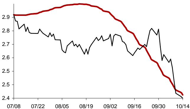
Chart 7: Forecast from Jul-08 2014 to Oct-14 2014
