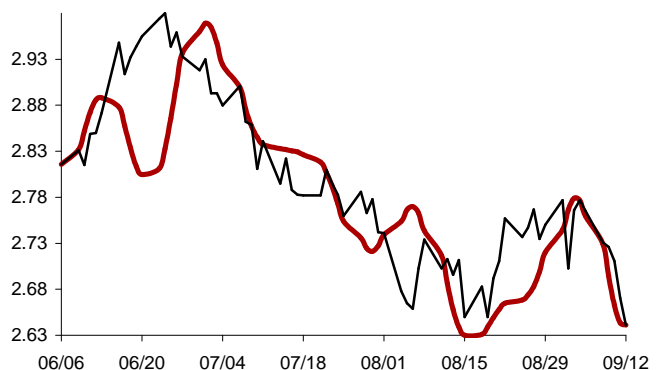
Chart 8: Forecast from Jun-06 2014 to Sep-12 2014
