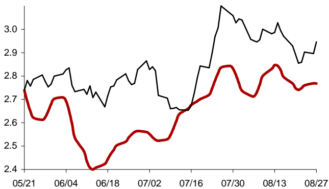
Chart 21: Forecast from May-21 2013 to Aug-27 2013
