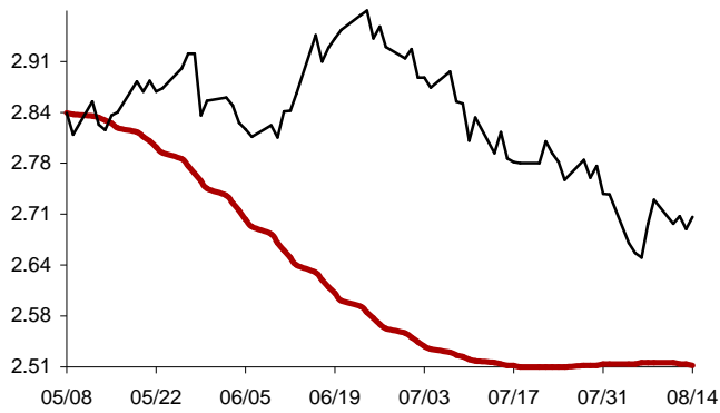
Chart 9: Forecast from May-08 2014 to Aug-14 2014
