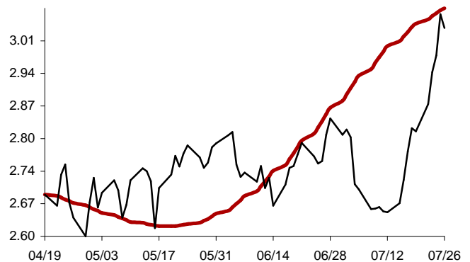
Chart 22: Forecast from Apr-19 2013 to Jul-26 2013
