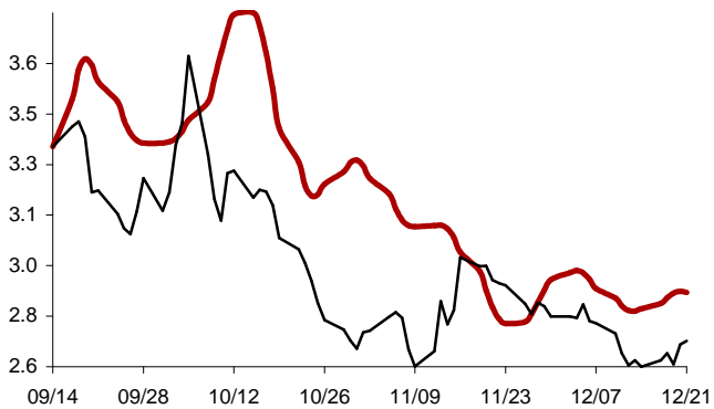
Chart 29: Forecast from Sep-14 2012 to Dec-21 2012
