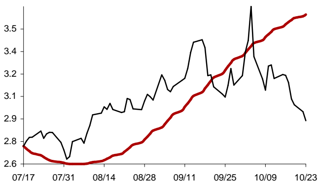
Chart 31: Forecast from Jul-17 2012 to Oct-23 2012
