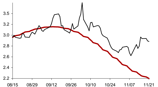
Chart 30: Forecast from Aug-15 2012 to Nov-21 2012
