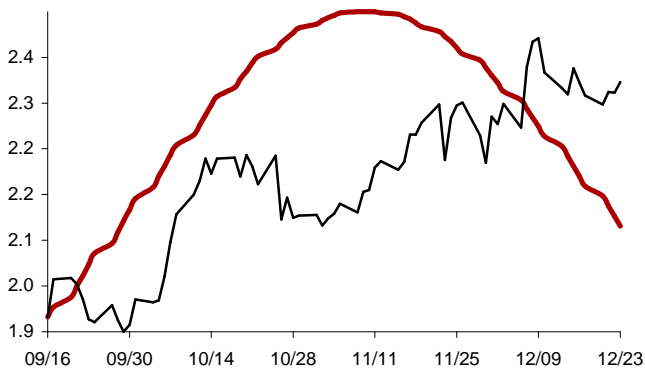
Chart 53: Forecast from Sep-03 2014 to Dec-10 2014
