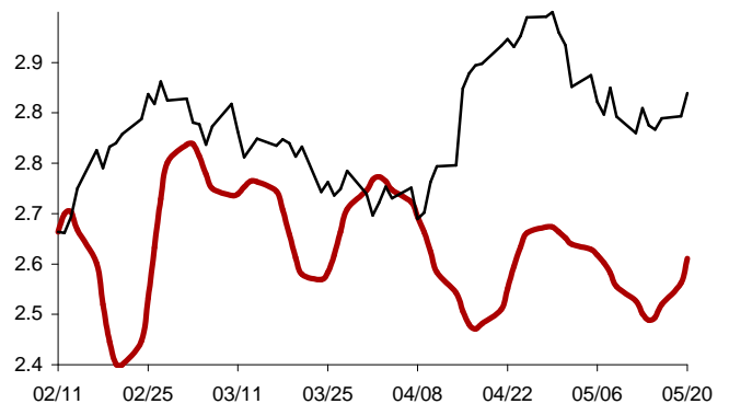
Chart 12: Forecast from Feb-12 2014 to May-20 2014
