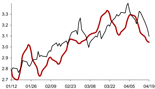
Chart 37: Forecast from Jan-12 2012 to Apr-19 2012
