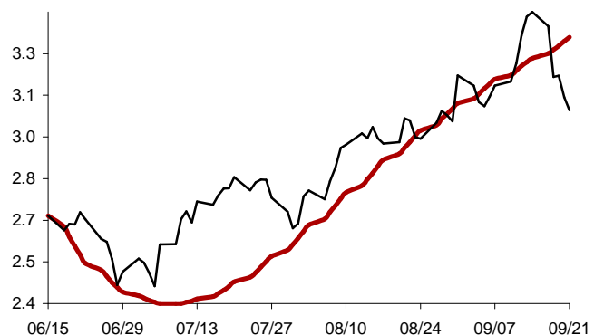
Chart 32: Forecast from Jun-15 2012 to Sep-21 2012
