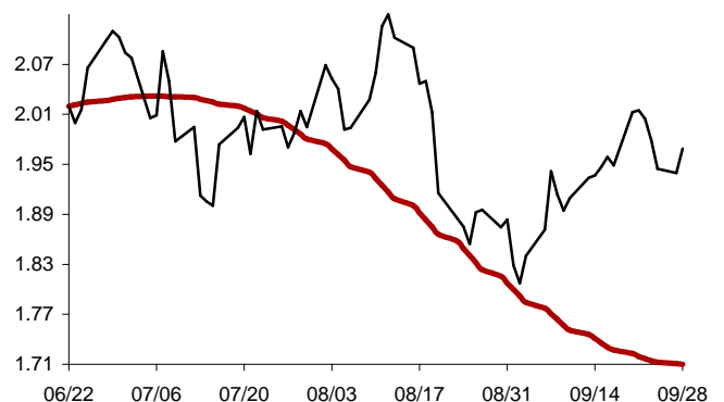
Chart 56: Forecast from Jun-06 2014 to Sep-12 2014
