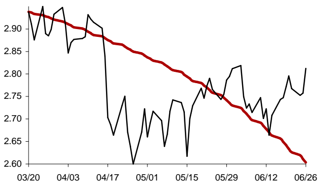
Chart 23: Forecast from Mar-20 2013 to Jun-26 2013
