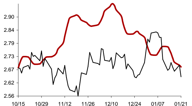
Chart 16: Forecast from Oct-15 2013 to Jan-21 2014
