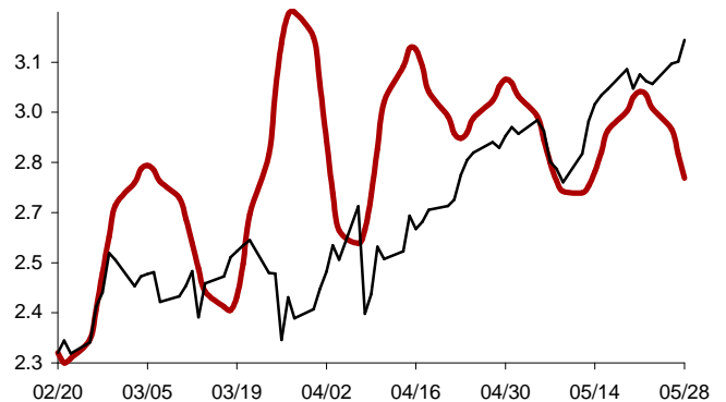
Chart 84: Forecast from Dec-03 2014 to Jan-08 2015
