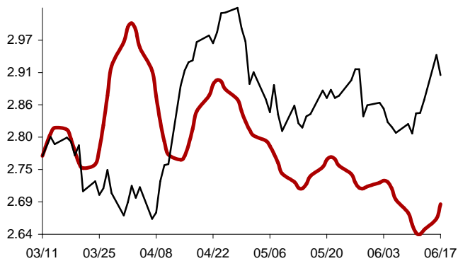
Chart 11: Forecast from Mar-11 2014 to Jun-17 2014
