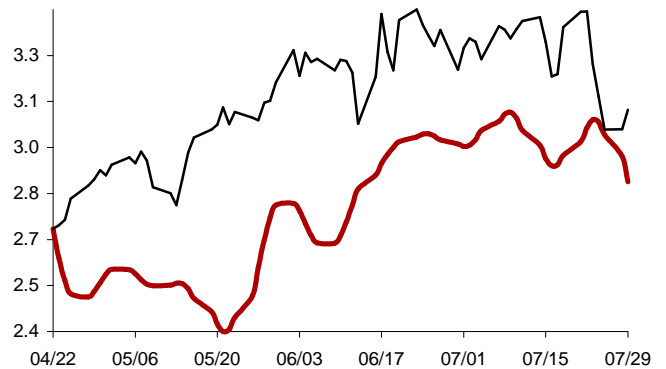
Chart 82: Forecast from Dec-02 2014 to Mar-10 2015
