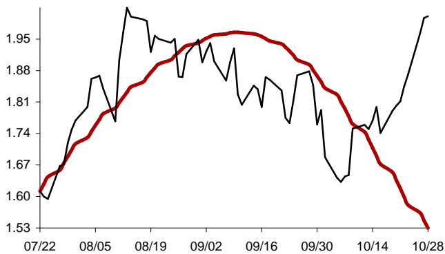
Chart 67: Forecast from Oct-31 2014 to Feb-06 2015
