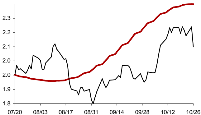
Chart 55: Forecast from Jul-08 2014 to Oct-14 2014
