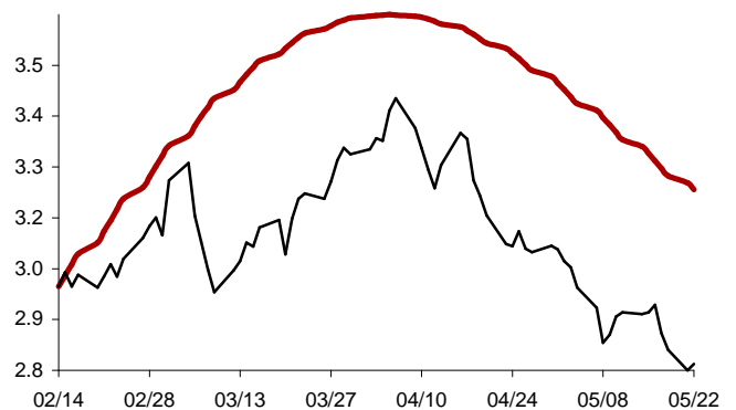
Chart 36: Forecast from Feb-15 2012 to May-22 2012
