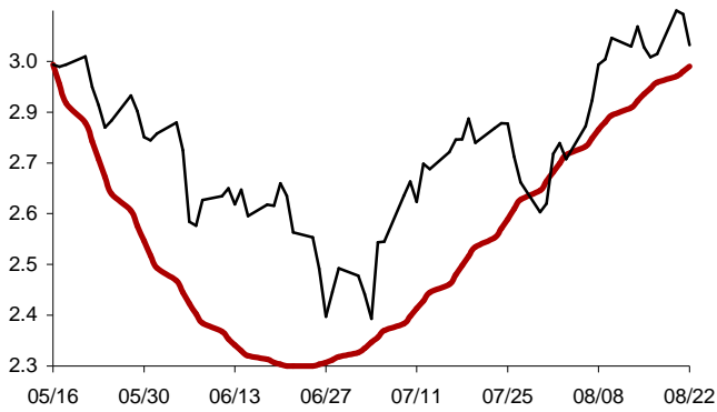
Chart 33: Forecast from May-16 2012 to Aug-22 2012
