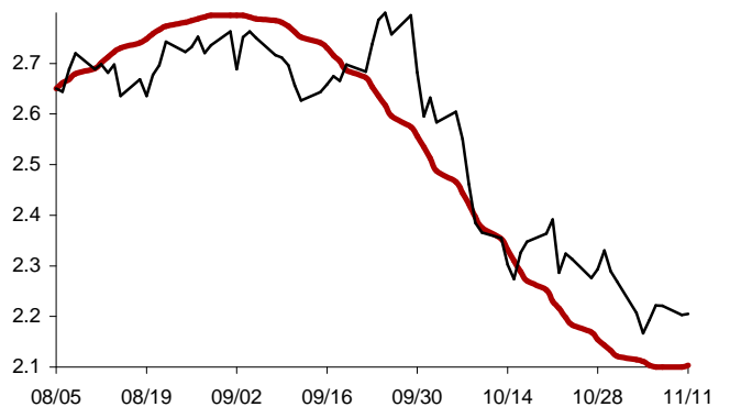
Chart 6: Forecast from Aug-05 2014 to Nov-11 2014
