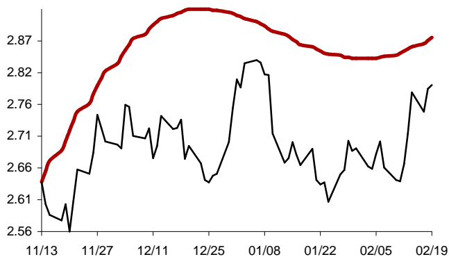
Chart 15: Forecast from Nov-13 2013 to Feb-19 2014
