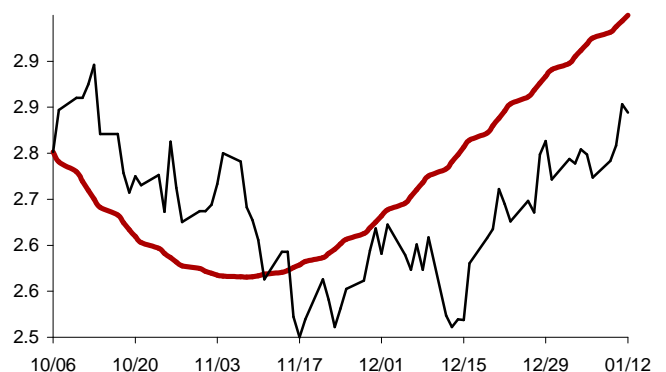
Chart 40: Forecast from Oct-06 2011 to Jan-12 2012
