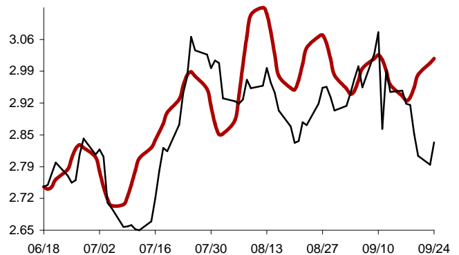
Chart 20: Forecast from Jun-19 2013 to Sep-24 2013
