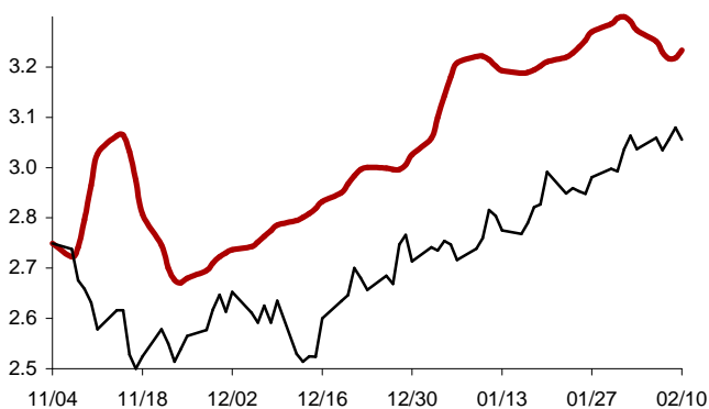
Chart 39: Forecast from Nov-04 2011 to Feb-10 2012
