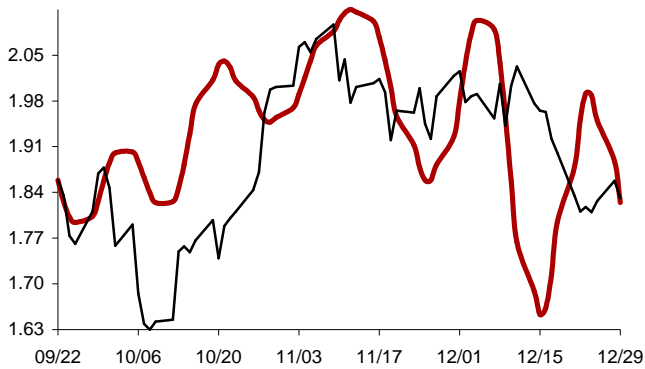
Chart 65: Forecast from Dec-31 2014 to Apr-08 2015
