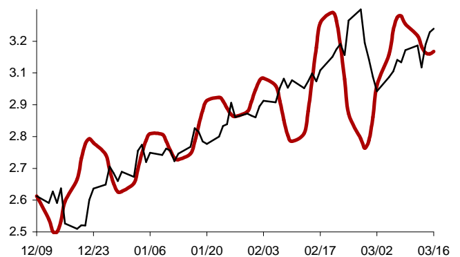
Chart 38: Forecast from Dec-09 2011 to Mar-16 2012
