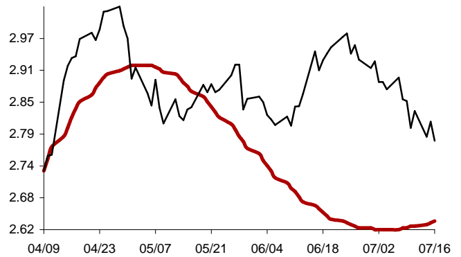
Chart 10: Forecast from Apr-09 2014 to Jul-16 2014
