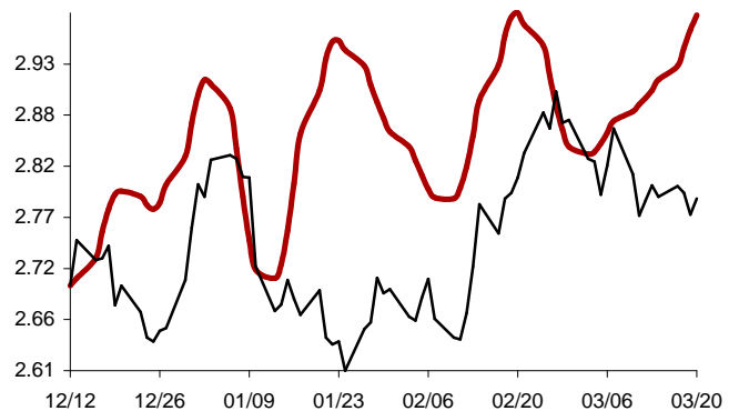
Chart 14: Forecast from Dec-12 2013 to Mar-20 2014
