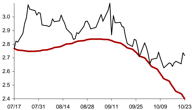
Chart 19: Forecast from Jul-17 2013 to Oct-23 2013
