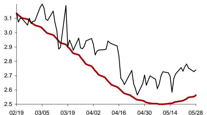
Chart 24: Forecast from Feb-19 2013 to May-28 2013
