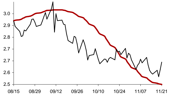
Chart 18: Forecast from Aug-15 2013 to Nov-21 2013
