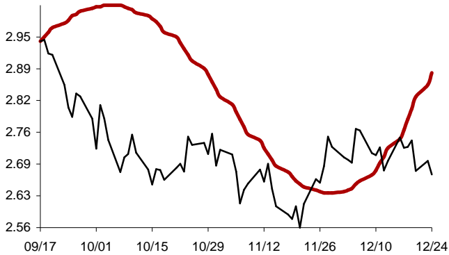
Chart 17: Forecast from Sep-17 2013 to Dec-24 2013
