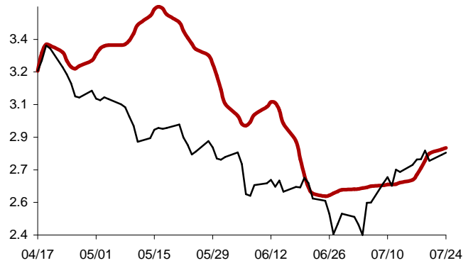
Chart 34: Forecast from Apr-17 2012 to Jul-24 2012
