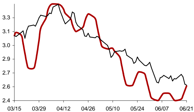
Chart 35: Forecast from Mar-15 2012 to Jun-21 2012
