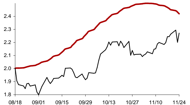
Chart 54: Forecast from Aug-05 2014 to Nov-11 2014
