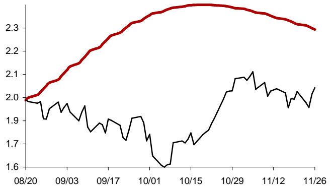
Chart 66: Forecast from Dec-02 2014 to Mar-10 2015
