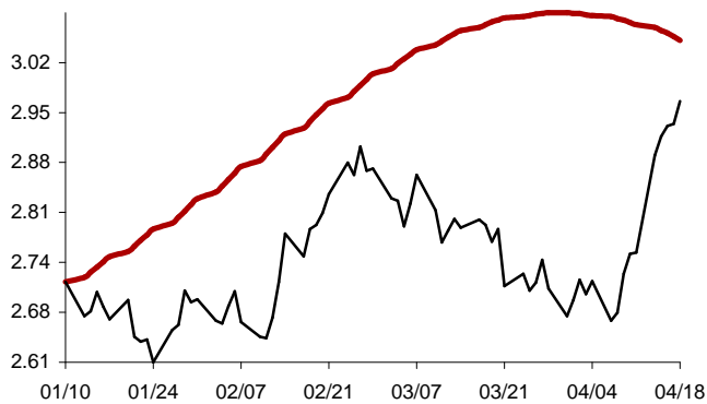
Chart 13: Forecast from Jan-10 2014 to Apr-18 2014
