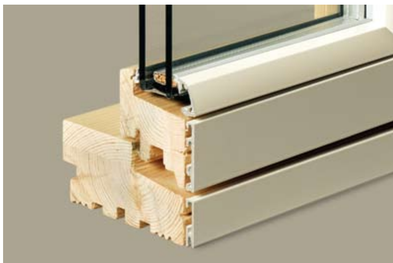
Laminated frame and sash & external aluminium cladding
