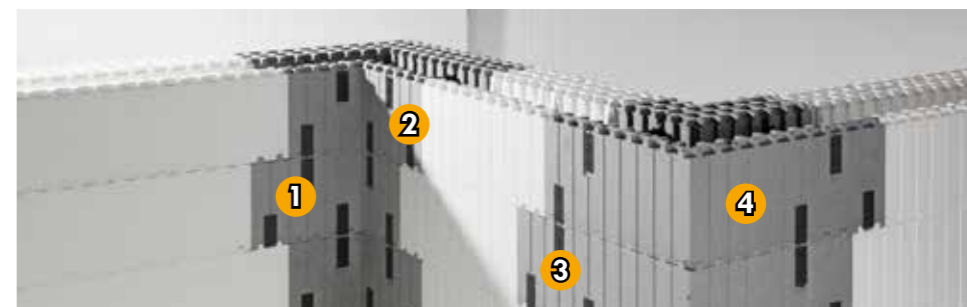
Schematic arrangement of corners (viewed from the inside of the building). Applied elements: 1 MCFU35 E90 LA, 2 MCFU35 E90 RA, 3 MCFU35 E90 LI, 4 MCFU35 E90 RI.
