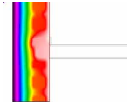
The MP ring beam element has an external insulation layer, which is the same as in the entire wall.
