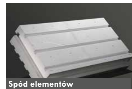
DPL GLT Above-rafter insulating panel (plain) 190x22x90 cm
