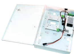
Paxton 12V 2A DC power supply - Metal cabinet
