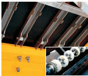
Agitation mechanism
