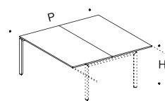
SCRIVANIE ACCOPIATE MULTIPLE CON GAMBE CENTRALI ARRETRATE MULTIPLE BACK-TO-BACK DESKS WITH CENTRALLY SPACED LEGS
