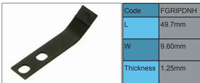
HEIDELBERG FEED BOARD - NO AIR HOLE
