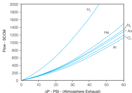
500 SCCM @ 30 psi N 2 Restrictor
