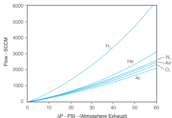
1000 SCCM @ 30 psi N 2 Restrictor
