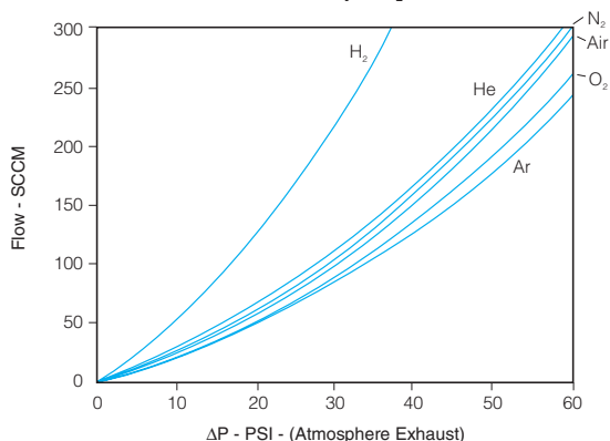
100 SCCM @ 30 psi N 2 Restrictor
